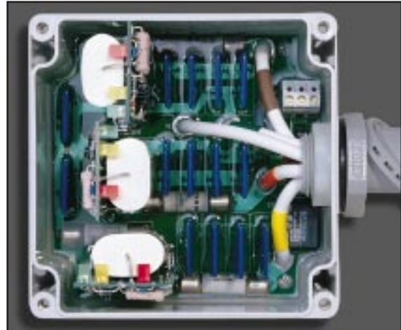
Regardless of surge capacity or voltage code, Model CPX systems are small in size and easy to install.
